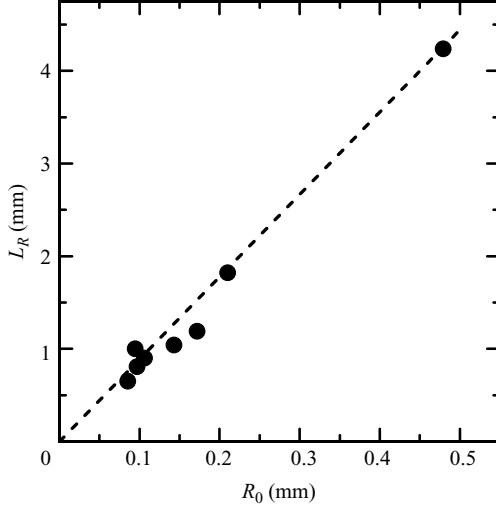
FIGURE 14. Wavelength of the beads observed on the jets in figure 1 as function of the jet radius. Dashed line: comparison with Rayleigh theory (3.30).
